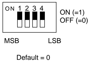
Figure 3-2, Card Address Switch
